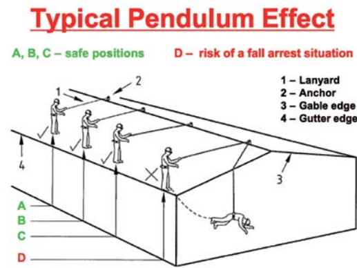
Limitations and dangers of using a restraint system on a sloping roof
